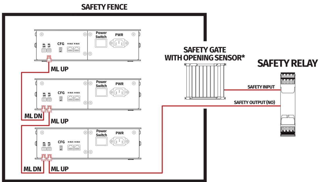
Example application of safety gate opening sensor:
